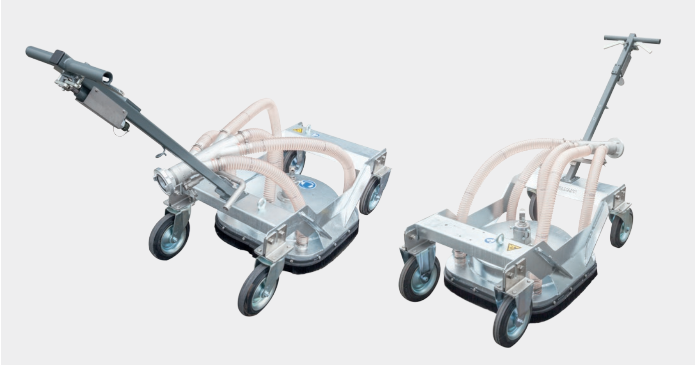
System with two steerable castors and two fixed castors for easy handling
